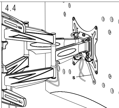
Level Adjustment
